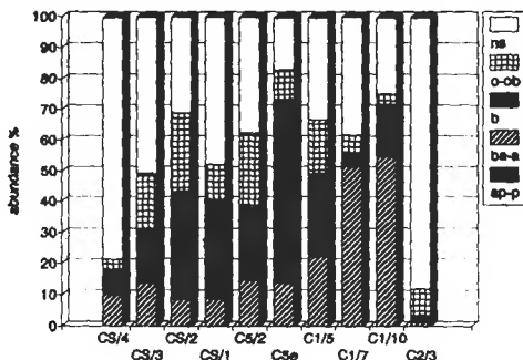
Fig. 6. Fig. 7. Percental distribution of ciliata species indicating different waterqualities within a population in spring 1991 and 1992 (ns=unknown indicative species, o-ob=oligo-oligobeta-mesosaprob sp., b=beta-mesosaprob sp., ba-a=beta-alfa-mesosaprob sp., ap-p=alfapoly-polysaprob sp.)
